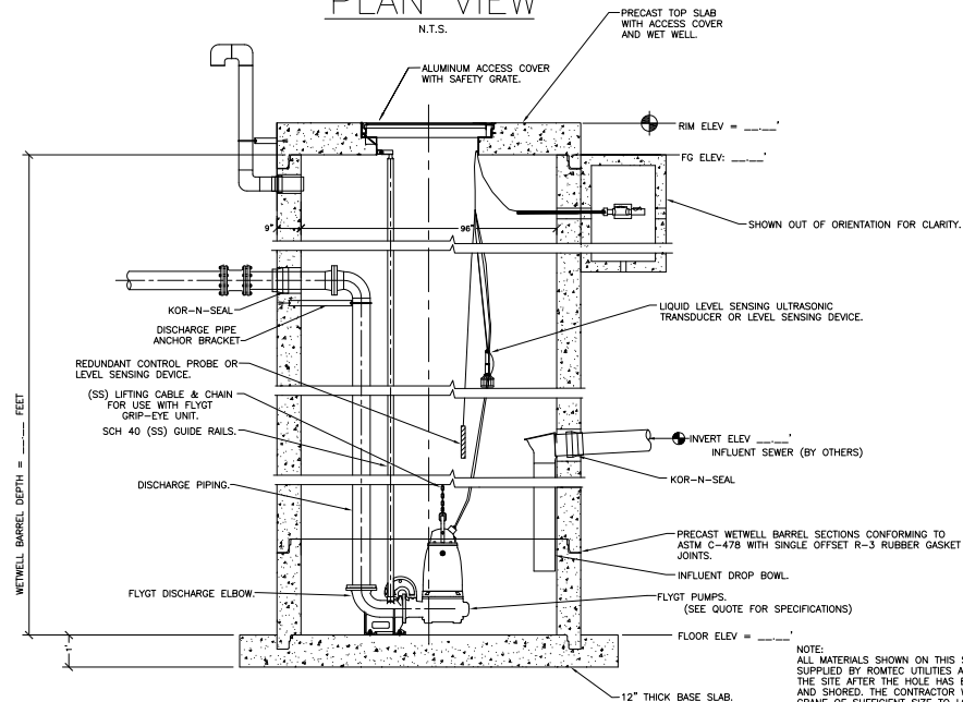
8' DIAMETER WETWELL SECTIONAL VIEW N.T.S.
